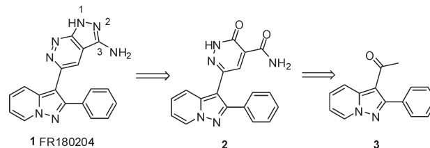
FIGURE 1. Retrosynthesis.
